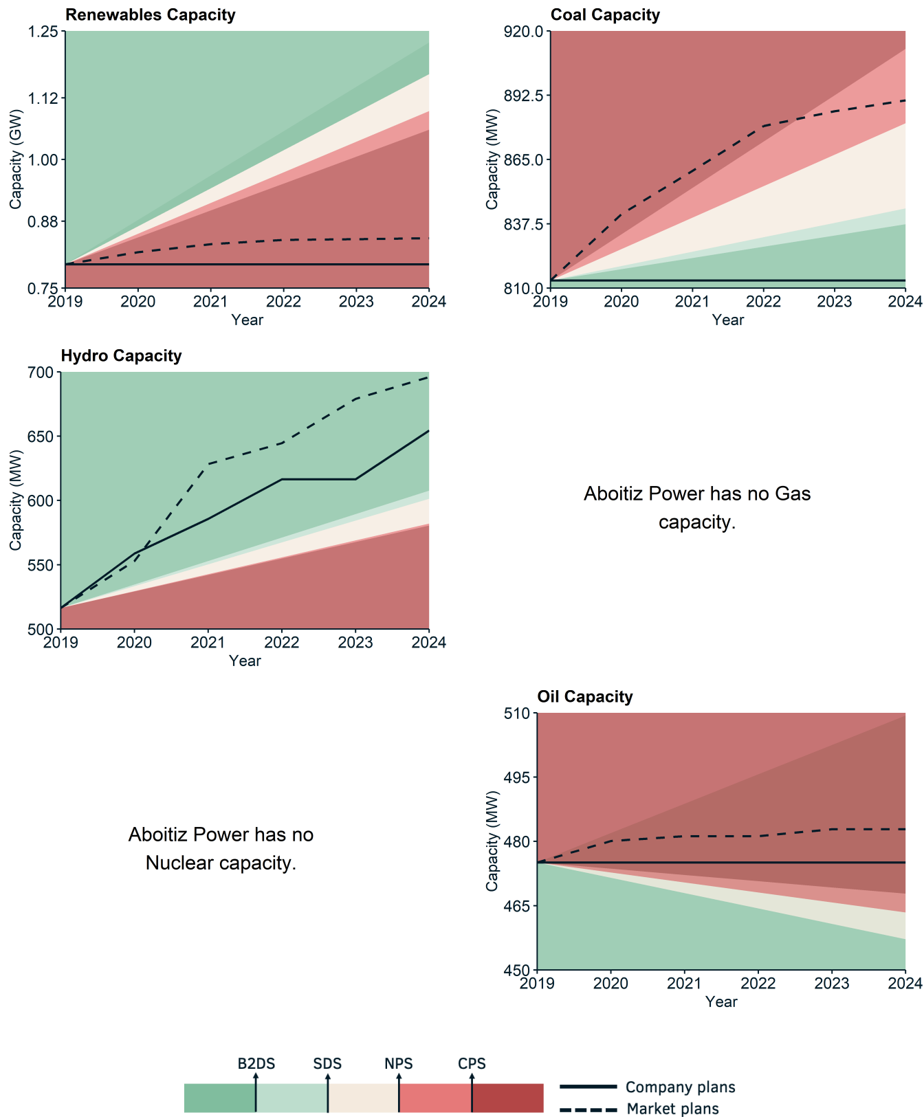
Figure 3.2: illustrates how Aboitiz Power's planned capacity changes in each technology compare to different IEA transition pathways and the market.
