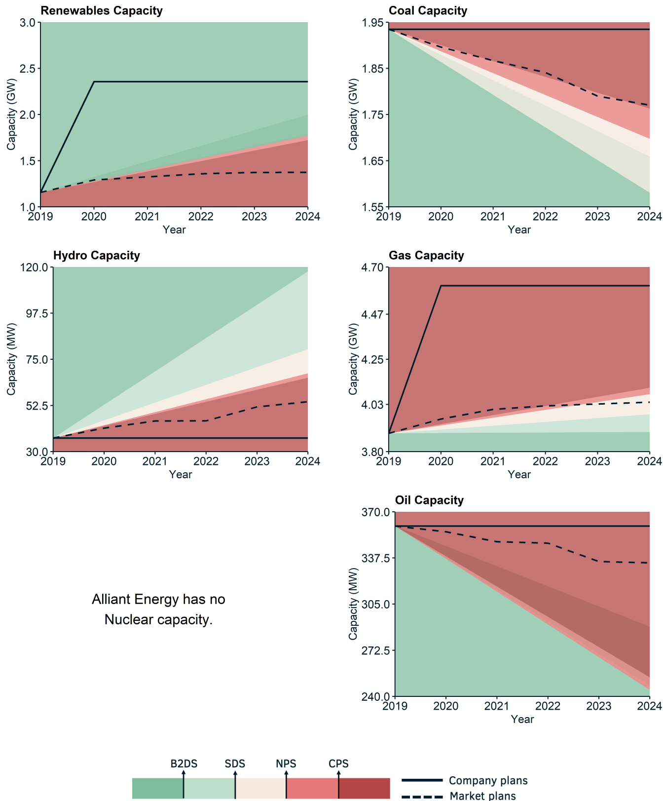
Figure 3.2: illustrates how Alliant Energy's planned capacity changes in each technology compare to different IEA transition pathways and the market.
