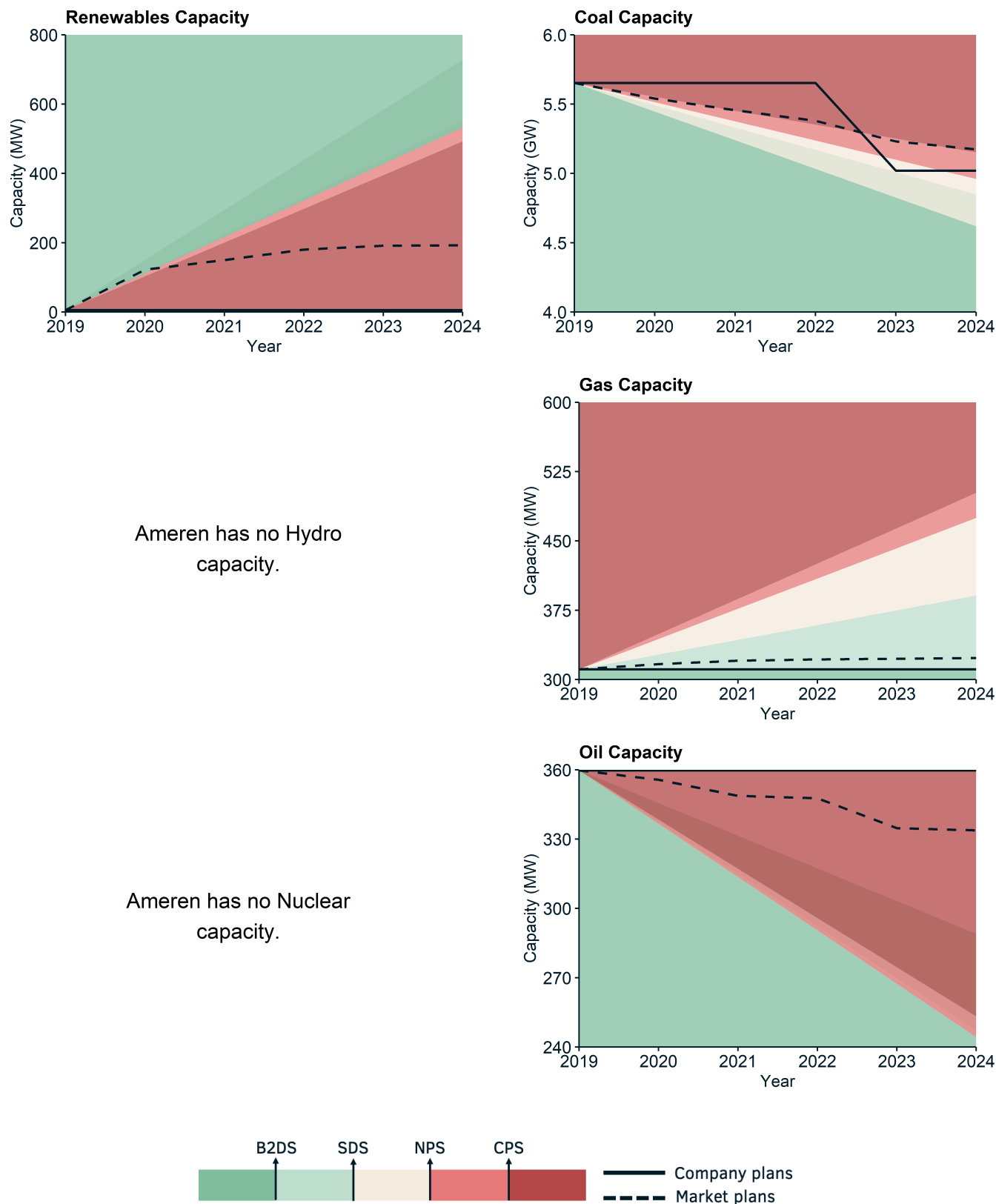
Figure 3.2: illustrates how Ameren's planned capacity changes in each technology compare to different IEA transition pathways and the market.
