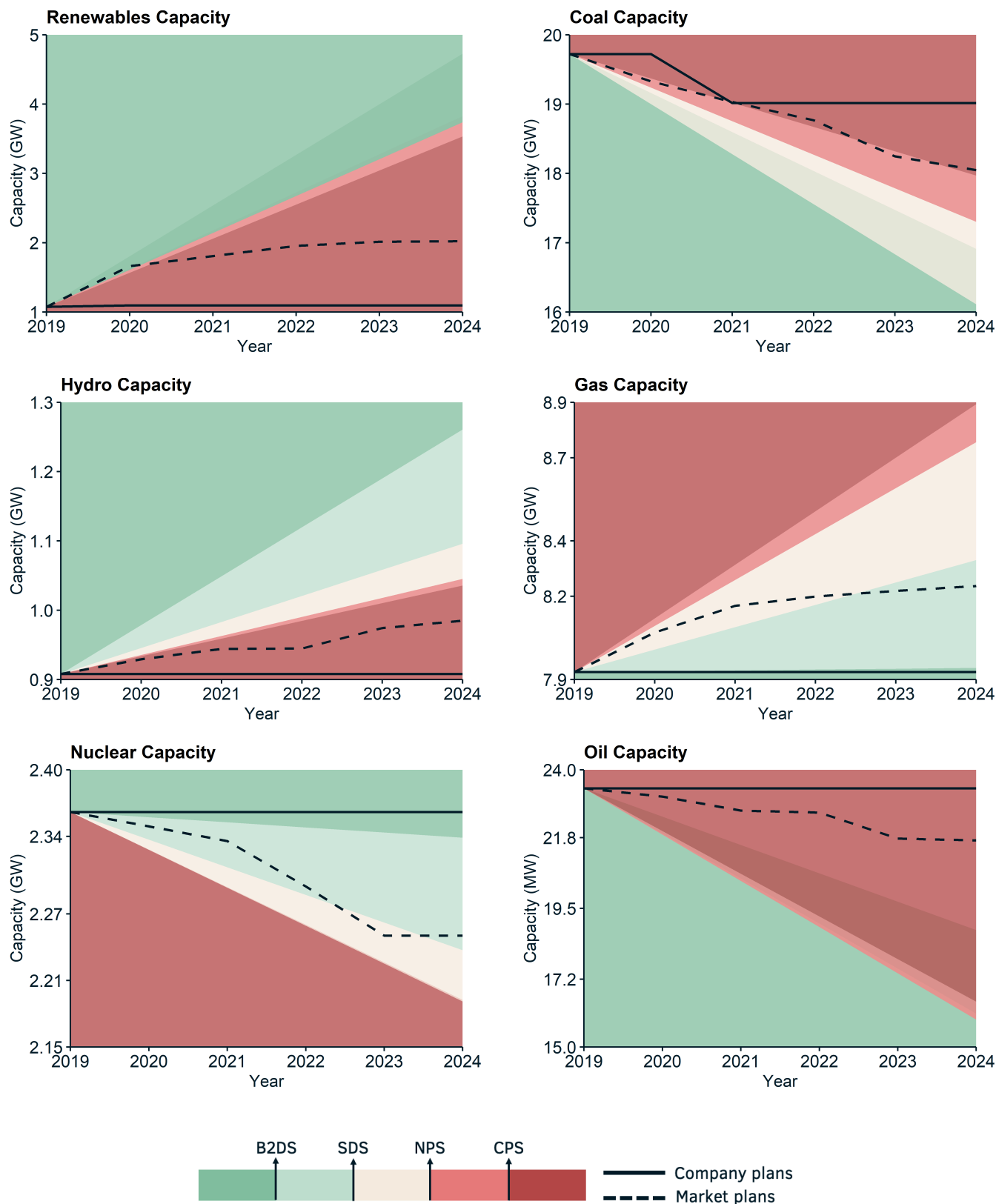
Figure 3.2: illustrates how AEP's planned capacity changes in each technology compare to different IEA transition pathways and the market.
