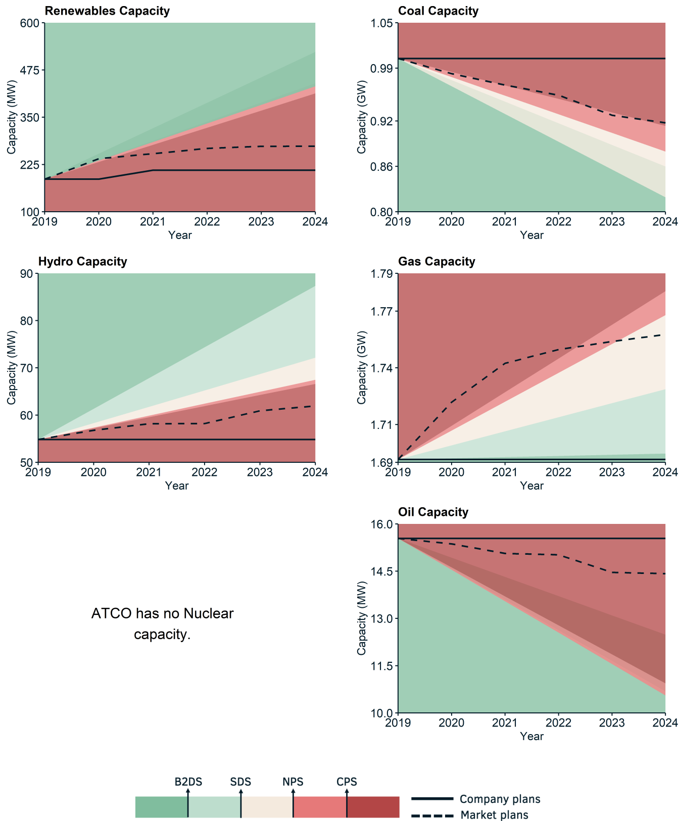
Figure 3.2: illustrates how ATCO's planned capacity changes in each technology compare to different IEA transition pathways and the market.
