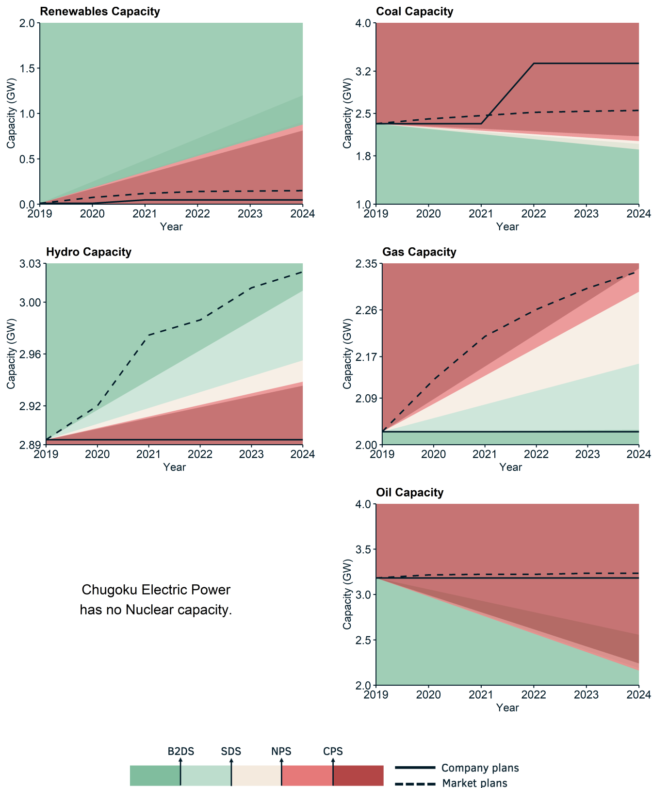
Figure 3.2: illustrates how Chugoku Electric Power's planned capacity changes in each technology compare to different IEA transition pathways and the market.
