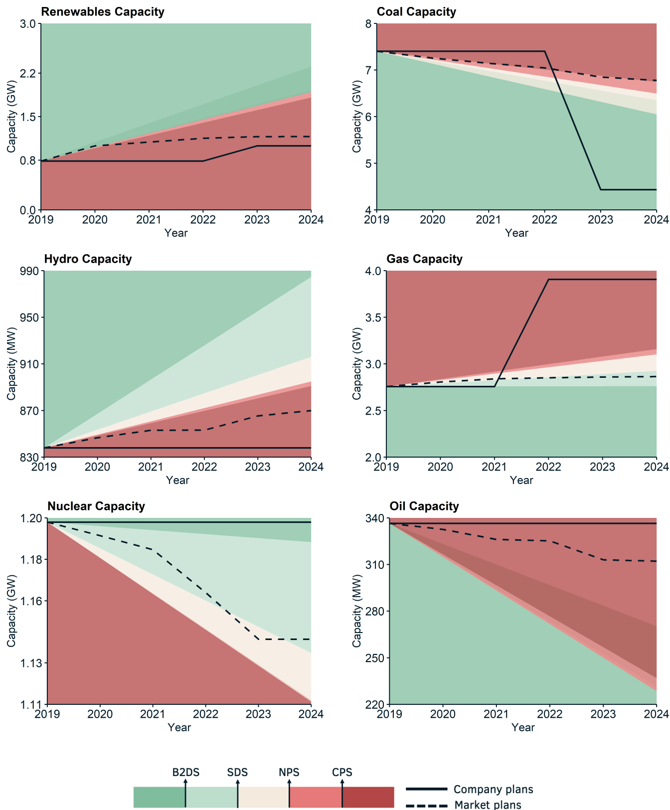
Figure 3.2: illustrates how DTE Energy's planned capacity changes in each technology compare to different IEA transition pathways and the market.
