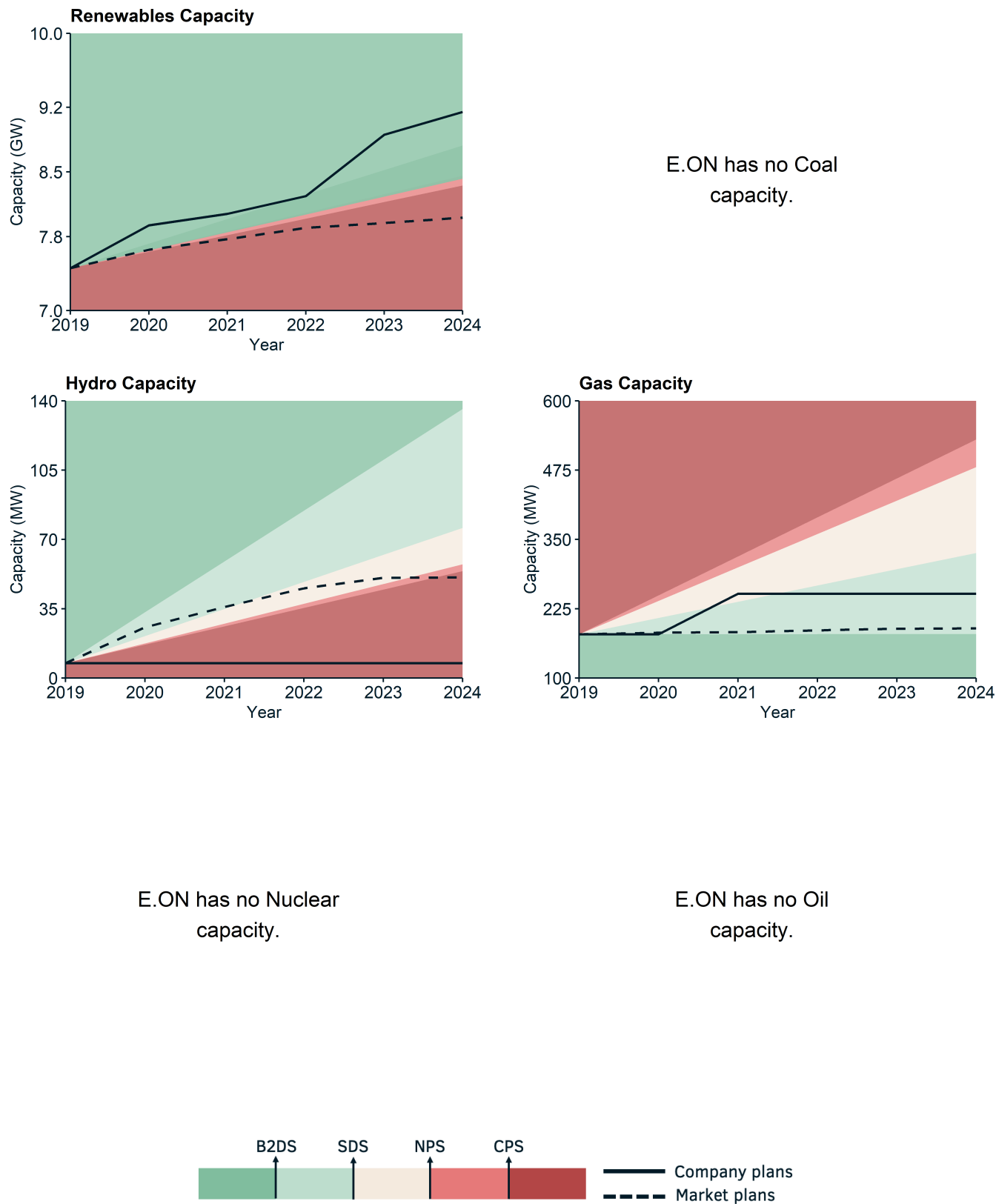
Figure 3.2: illustrates how E.ON's planned capacity changes in each technology compare to different IEA transition pathways and the market.
