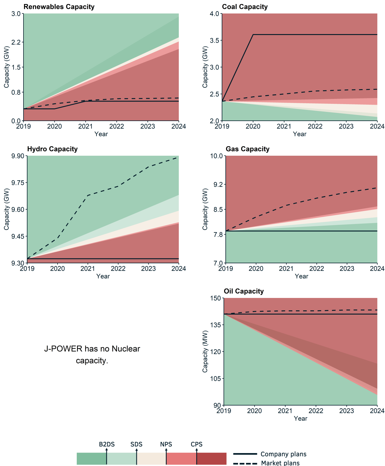
Figure 3.2: illustrates how J-POWER's planned capacity changes in each technology compare to different IEA transition pathways and the market.
