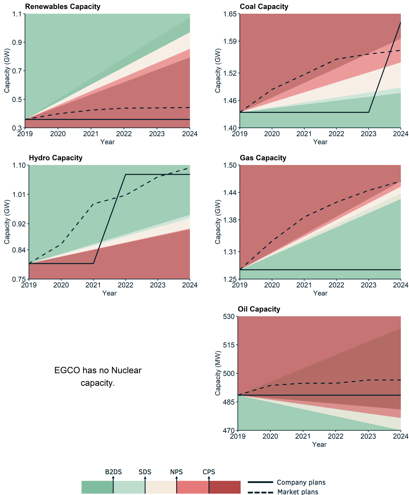
Figure 3.2: illustrates how EGCO's planned capacity changes in each technology compare to different IEA transition pathways and the market.
