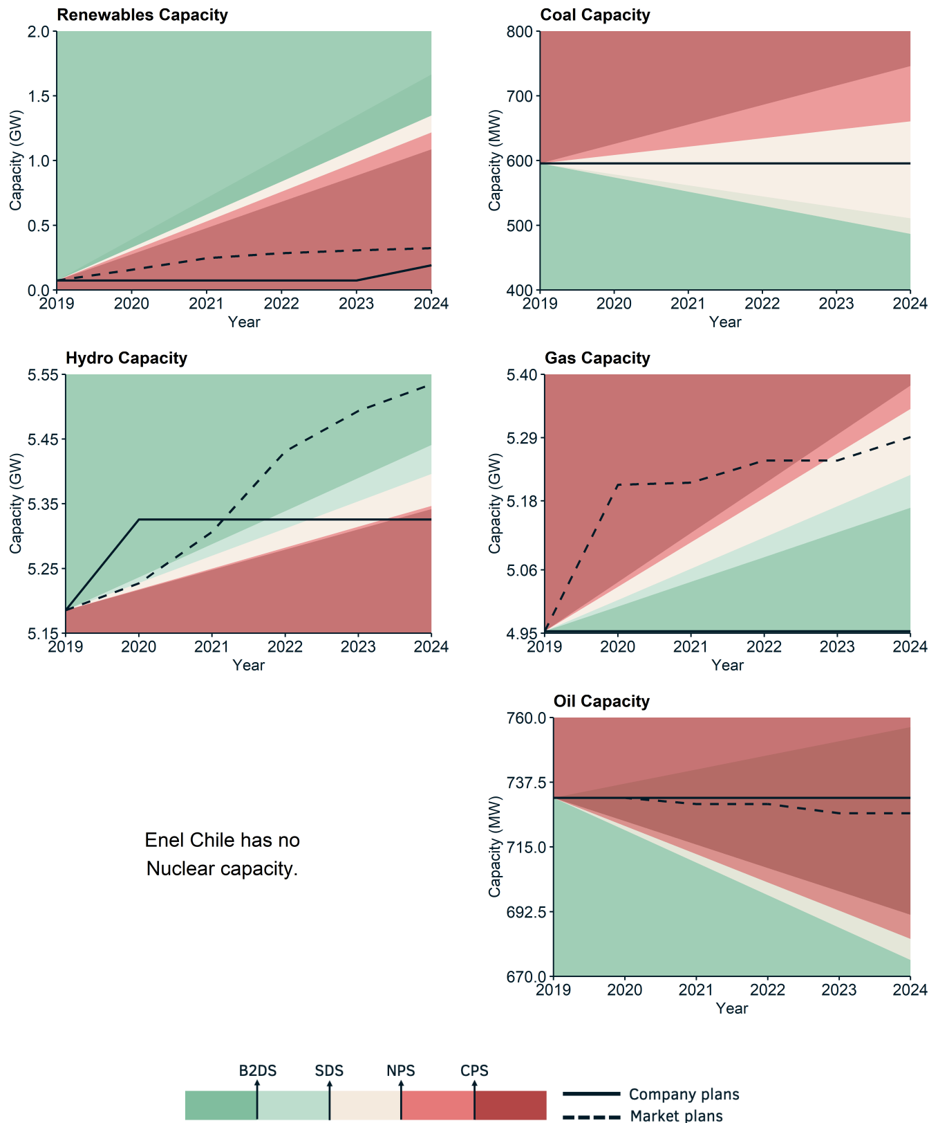
Figure 3.2: illustrates how Enel Chile 's planned capacity changes in each technology compare to different IEA transition pathways and the market.
