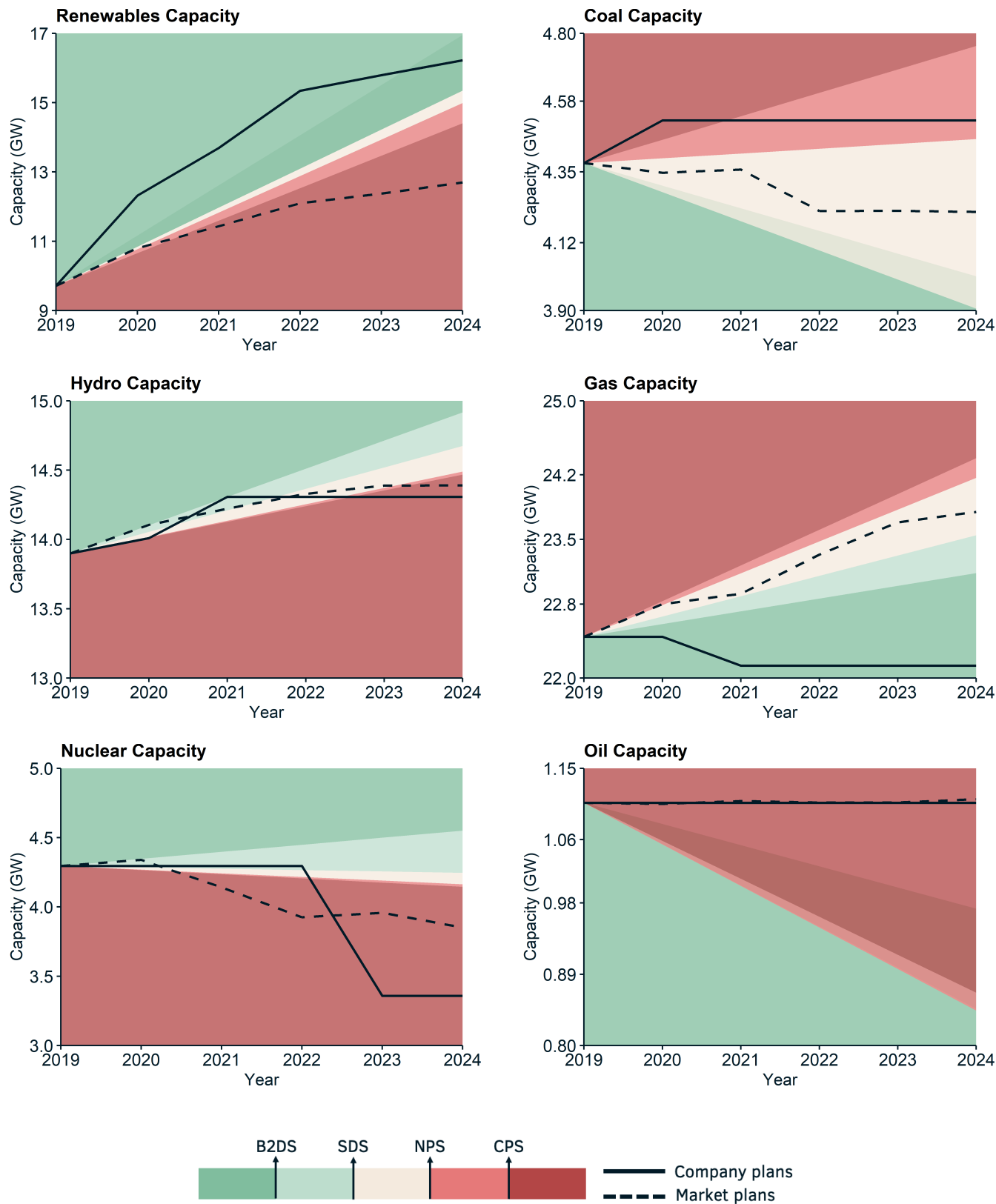
Figure 3.2: illustrates how ENGIE's planned capacity changes in each technology compare to different IEA transition pathways and the market.
