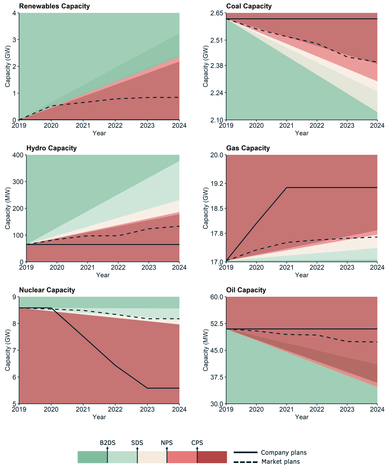
Figure 3.2: illustrates how Entergy's planned capacity changes in each technology compare to different IEA transition pathways and the market.
