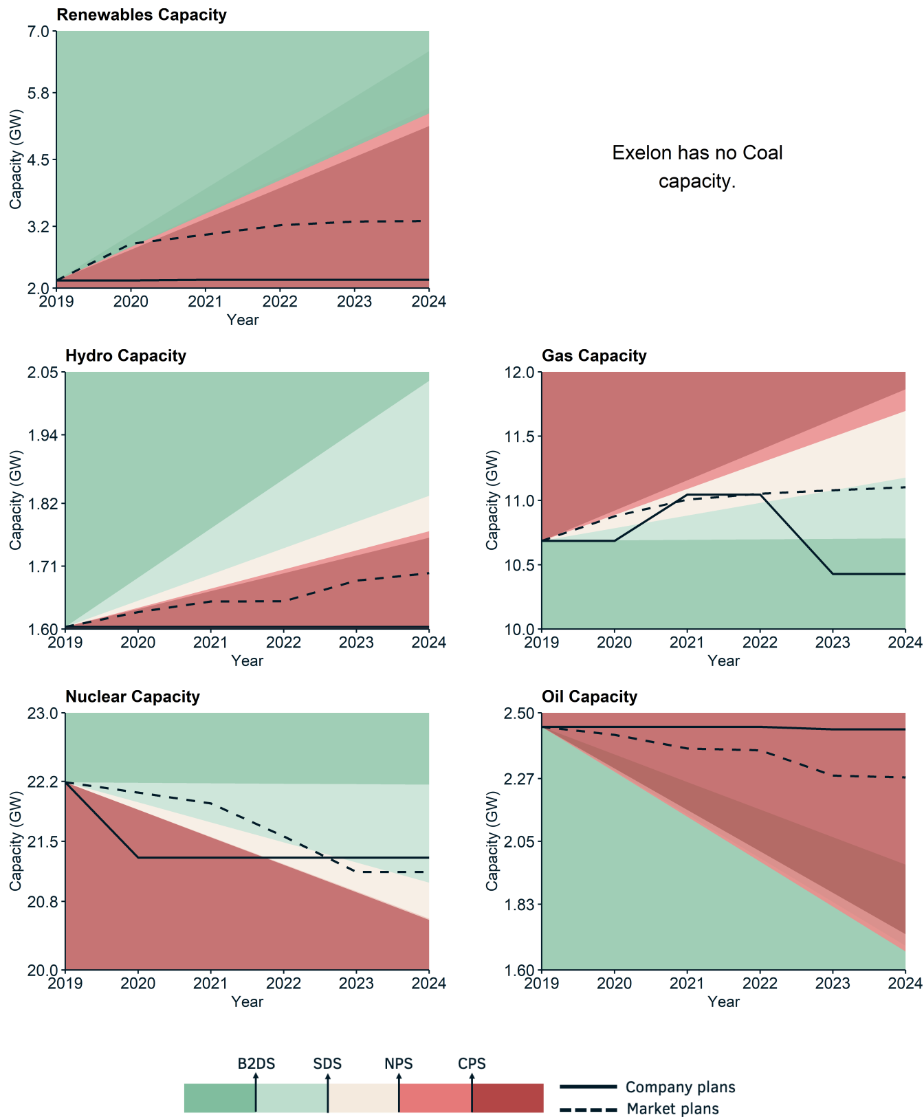
Figure 3.2: illustrates how Exelon's planned capacity changes in each technology compare to different IEA transition pathways and the market.
