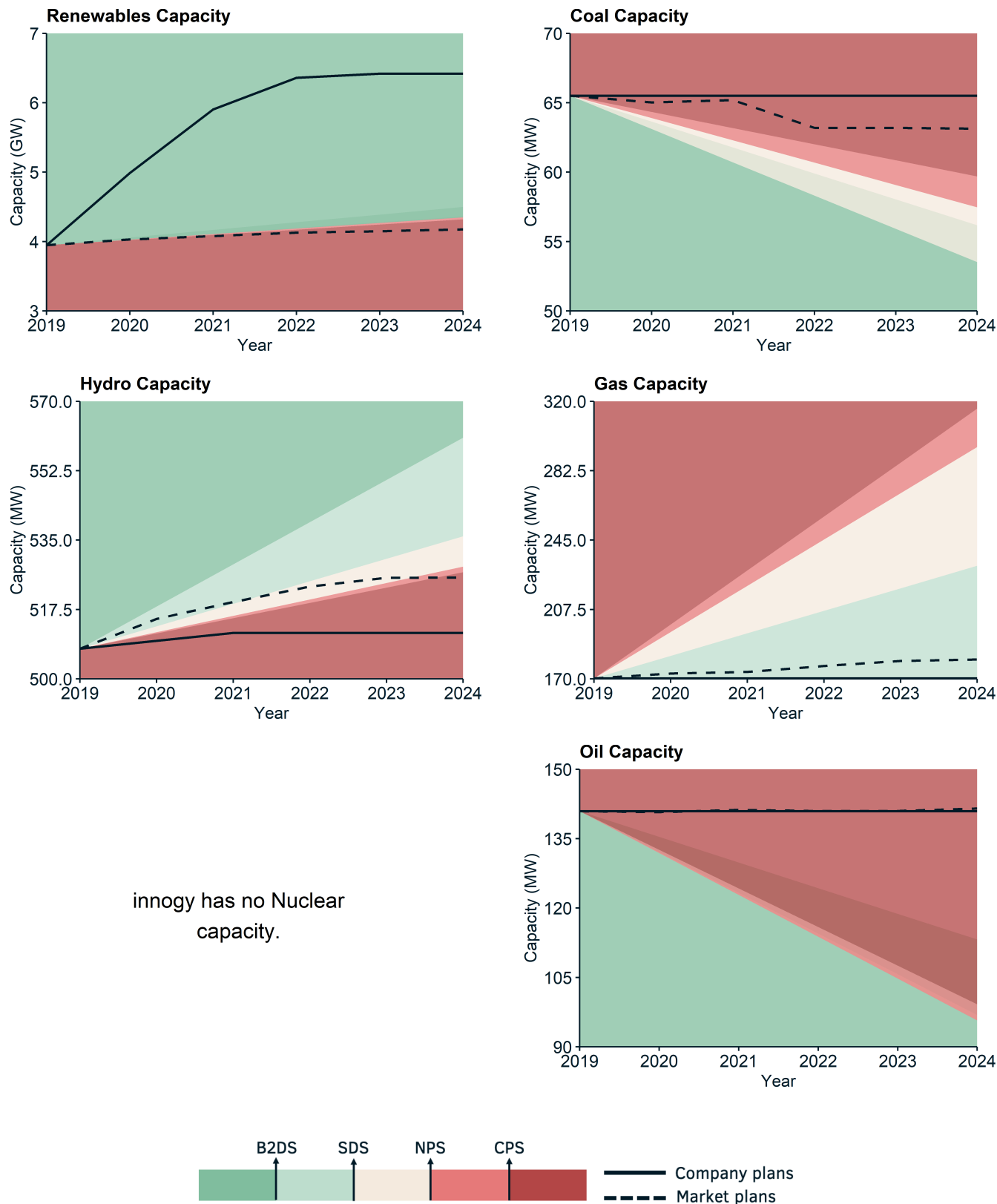
Figure 3.2: illustrates how innogy's planned capacity changes in each technology compare to different IEA transition pathways and the market.
