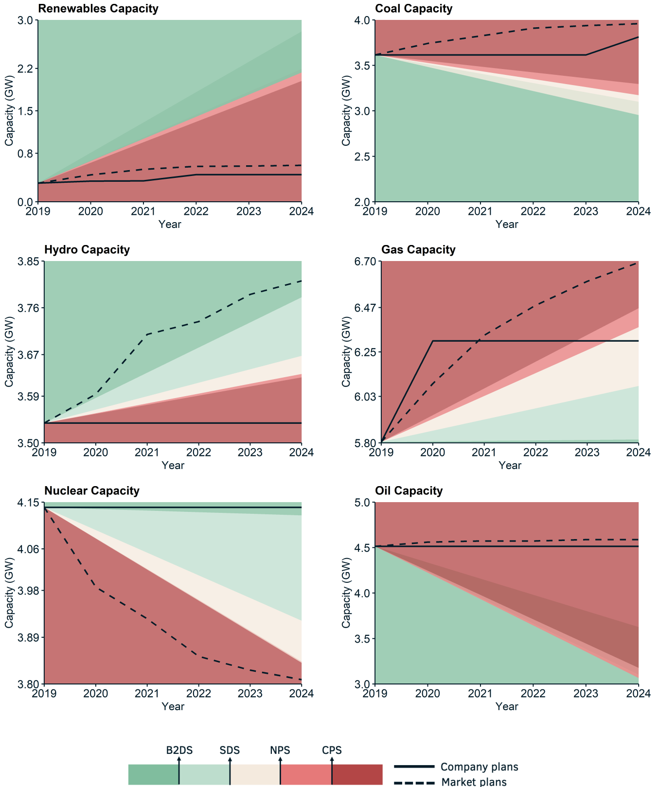
Figure 3.2: illustrates how Kyushu Electric Power's planned capacity changes in each technology compare to different IEA transition pathways and the market.
