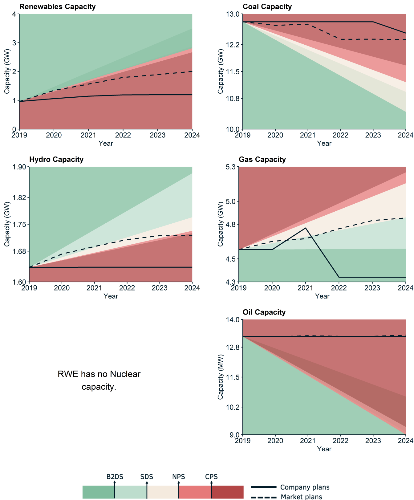
Figure 3.2: illustrates how RWE's planned capacity changes in each technology compare to different IEA transition pathways and the market.
