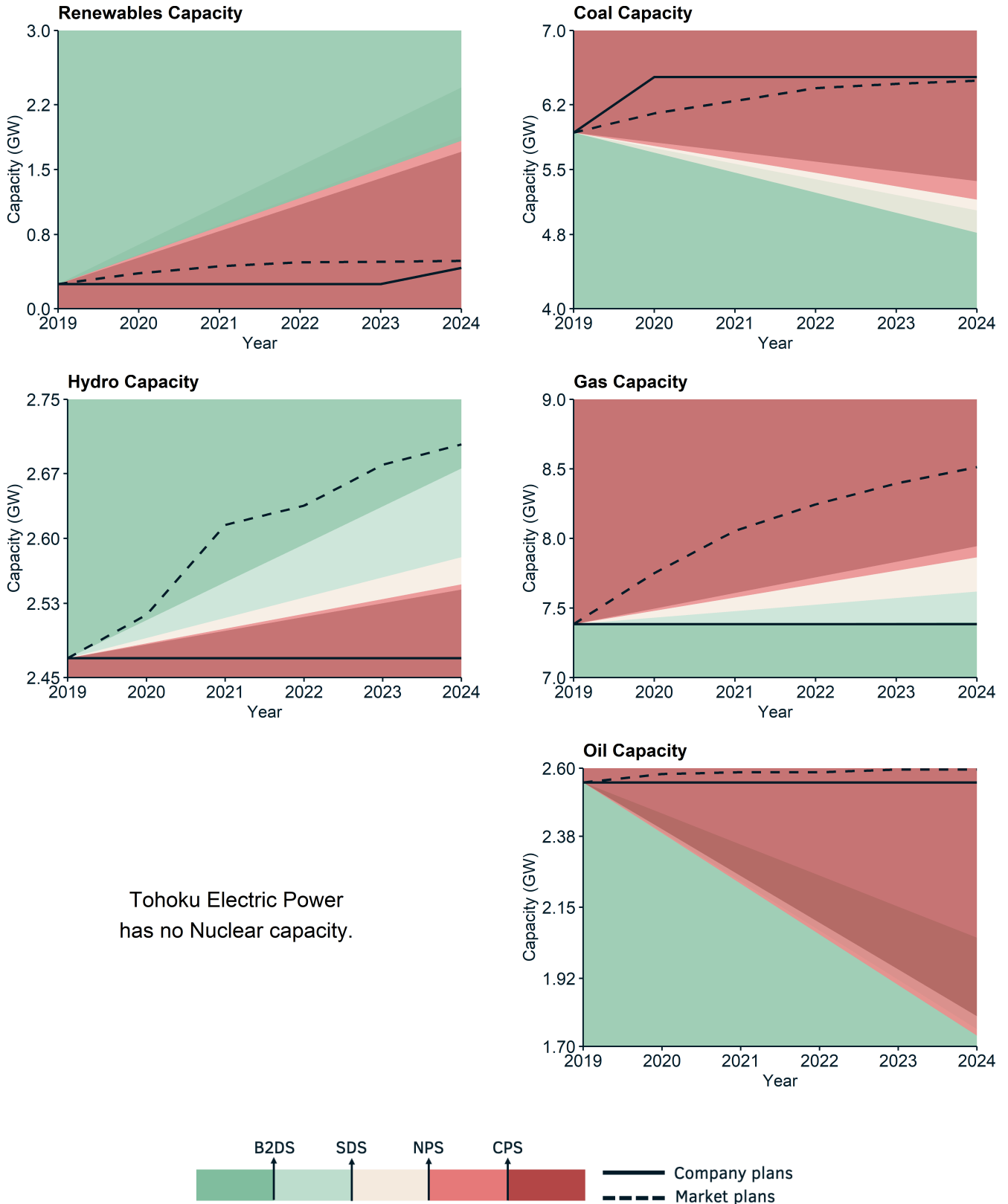
Figure 3.2: illustrates how Tohoku Electric Power's planned capacity changes in each technology compare to different IEA transition pathways and the market.
