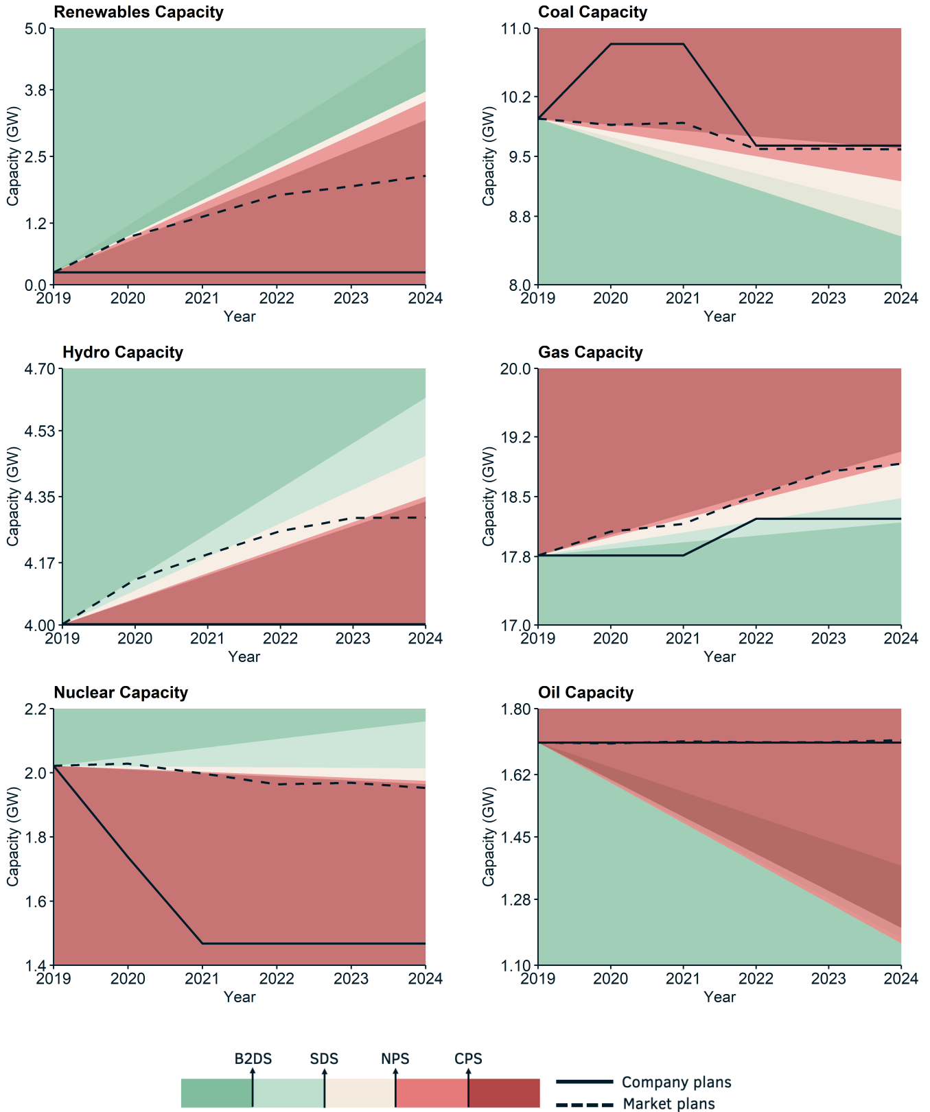
Figure 3.2: illustrates how Uniper's planned capacity changes in each technology compare to different IEA transition pathways and the market.
