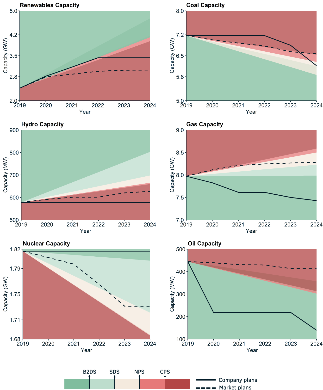
Figure 3.2: illustrates how Xcel Energy's planned capacity changes in each technology compare to different IEA transition pathways and the market.
