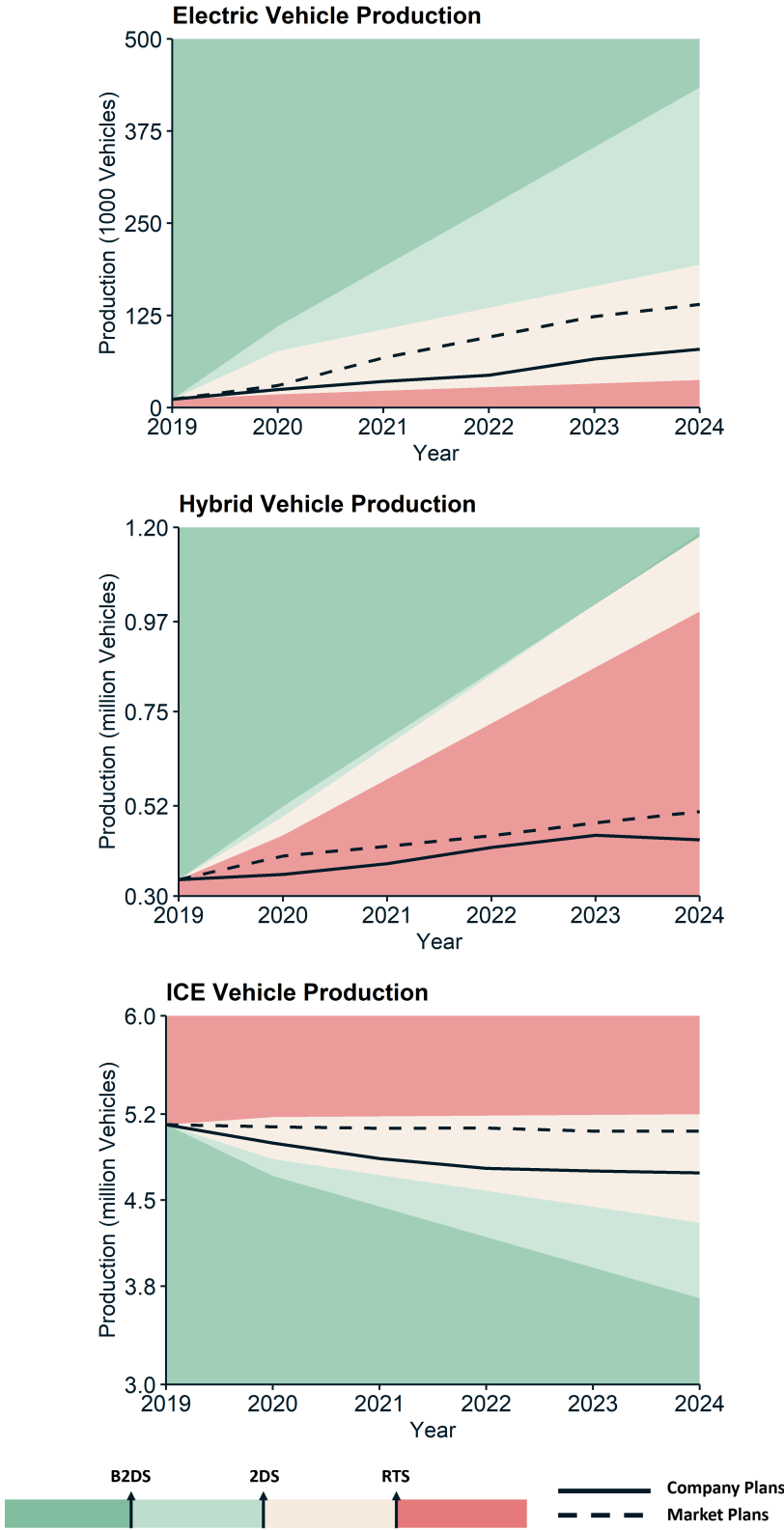
Figure 3.2: illustrates how Honda's planned production changes in each technology compare to different IEA transition pathways and the market.
