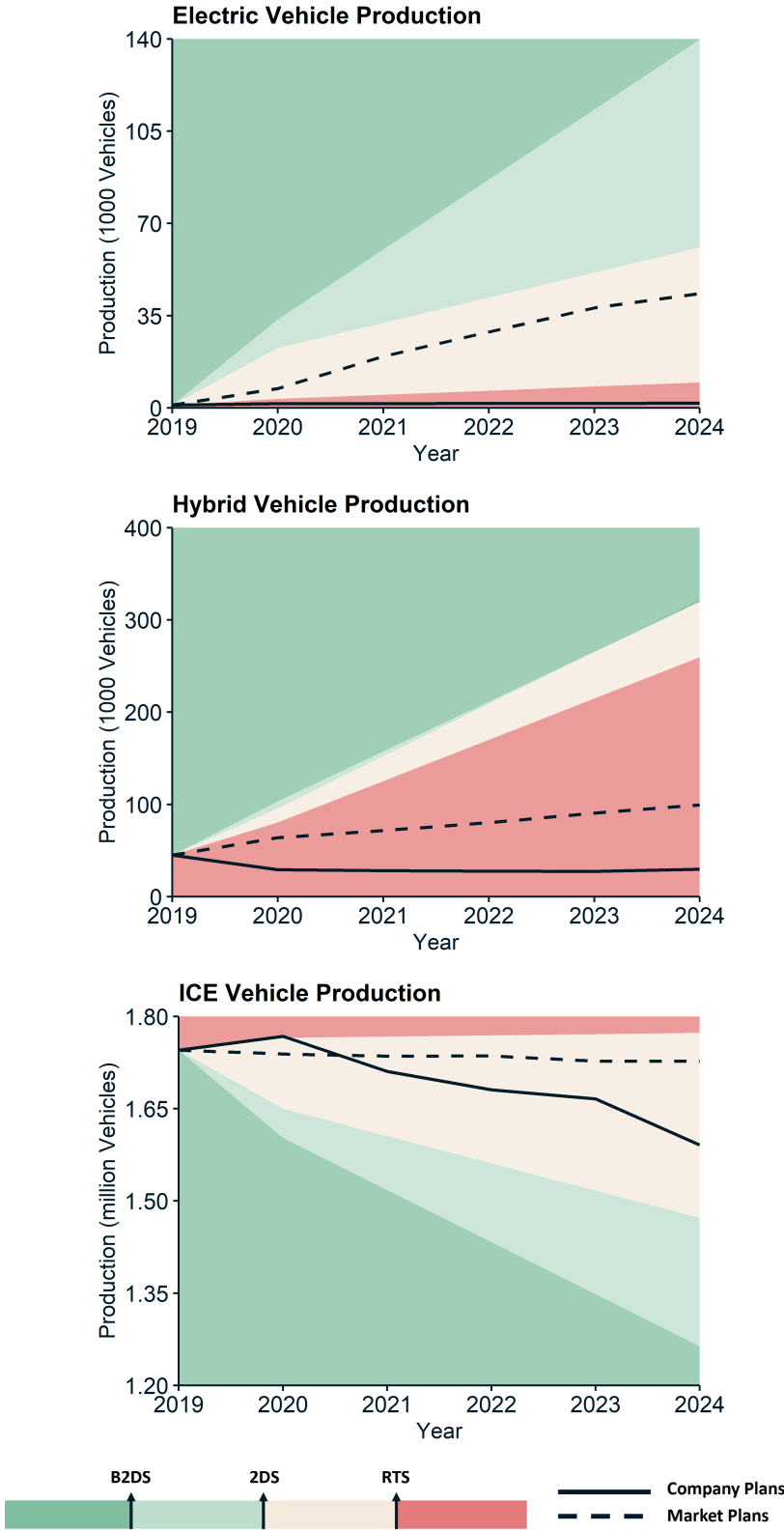
Figure 3.2: illustrates how Maruti Suzuki India Ltd's planned production changes in each technology compare to different IEA transition pathways and the market.
